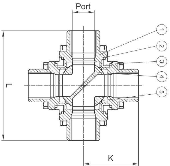
4 WAY "L"(X)PORT
